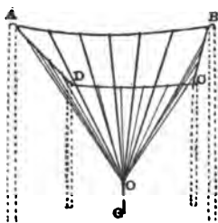
FIG. 30.—Type of Inverted Cone Antenna.
